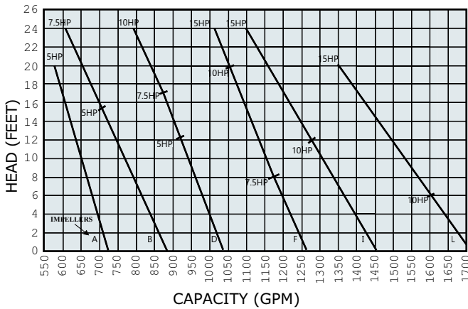
AF06 PUMP CURVES
